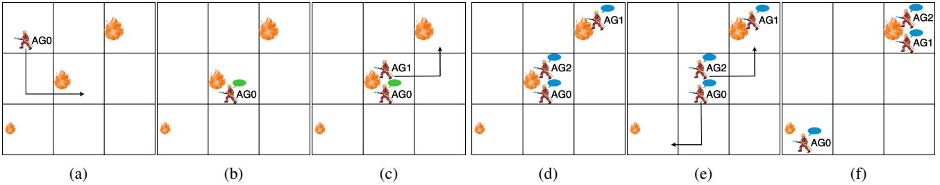
Fig. 2: A complete episode of the Urban Firefighting domain with learned oDec-AIRL policies. Colored bubbles green and blue represent CallAgent and Extinguish actions respectively. In Figure 2a, Agent 0 heads towards the medium fire, and Figure 2b, calls Agent 1 to join. Subsequently, Agent 1 moves to the large fire in Figure 2c, while Agent 0 calls Agent 2. In Figure 2d, all agents extinguish fires at their locations. After extinguishing the medium fire, Agent 0 moves to the small fire, and Agent 2 assists Agent 1 with the large fire in Figure 2e. Figure 2f shows agents at their final locations performing the Extinguish action. This visualization was built using PyGame [14].
