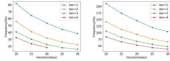
Fig. 7. Time Performance of iLQGame and MPPI-IBR.
