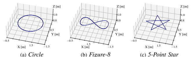
Fig. 4: The Circle , Figure-8 and 5-Point Star reference trajectories, with periods of 3 s, 5 s and 6 s respectively. All trajectories lie in the horizontal xy-plane 1 m above the ground, and start at the point (0, 0, 1) m.
